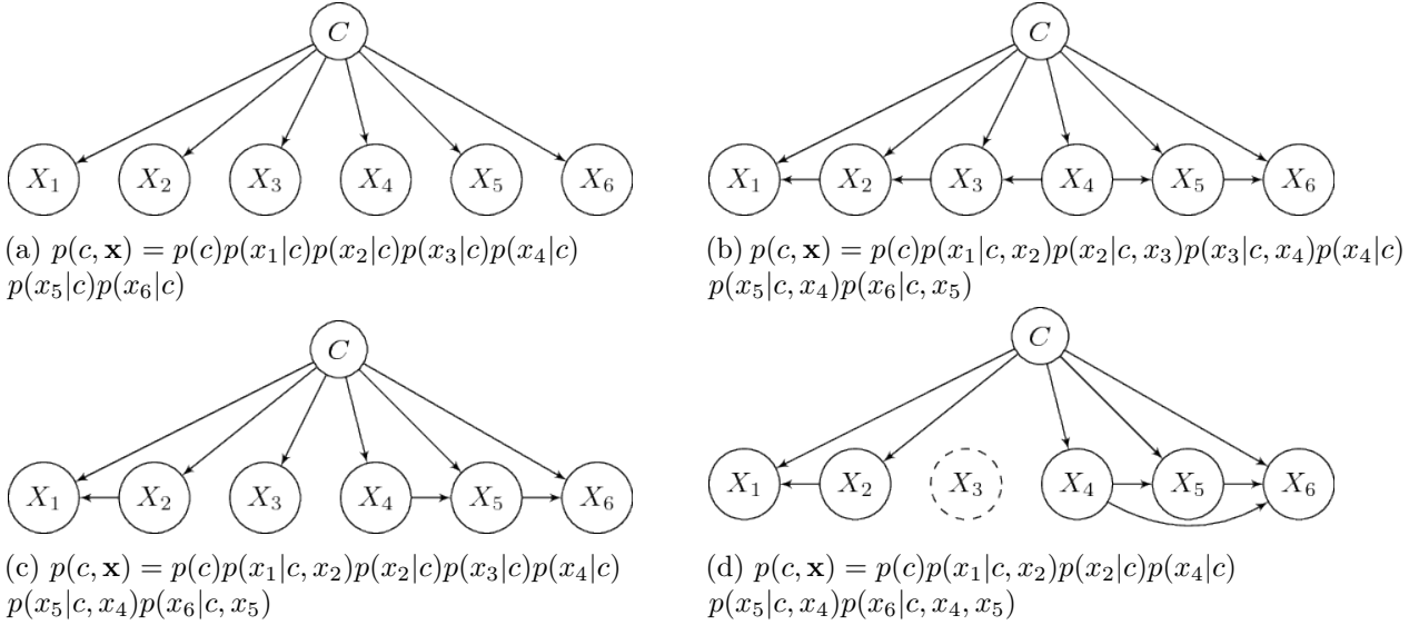
Figure 1: Augmented naive Bayes models produced by the bnlearn package. (a) NB; (b) TAN (c) FAN (d) SNB. k-DB and AODE not shown. The NB assumes that the features are independent given the class. ODE allows each predictor to depend on at most one other predictor: the TAN is a special case with exactly n - 1 augmenting arcs (i.e., inter-feature arcs) while a FAN may have less than n - 1 . The k-DB allows for up to k parent features per feature X_i , with NB and ODE as its special cases with k = 0 and k = 1 , respectively. The SNB does not restrict the number of parents but requires that connected feature subgraphs be complete (connected, after removing C , subgraphs in (d): \{X_1, X_2\} , and \{X_4, X_5, X_6\} ), also allowing the removal of features ( X_3 omitted in (d)). The AODE is not a single structure but an ensemble of n ODE models in which one feature is the parent of all others (a super-parent).
